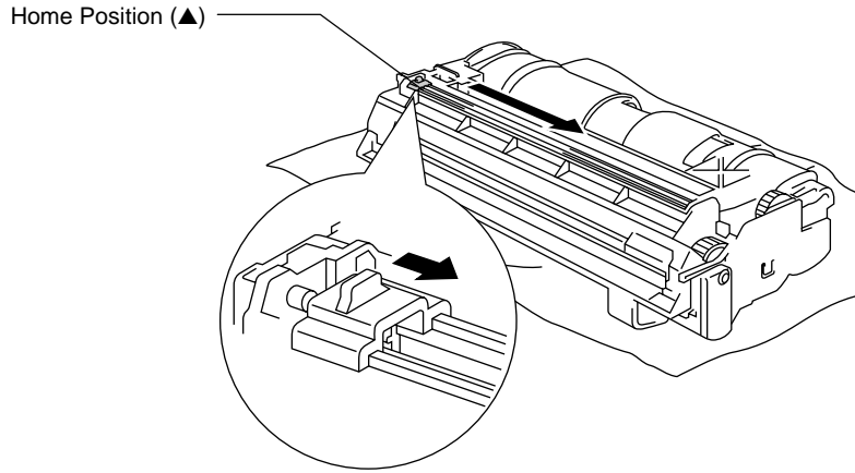
Fig. 6-9 Cleaning the Primary Corona Wire
